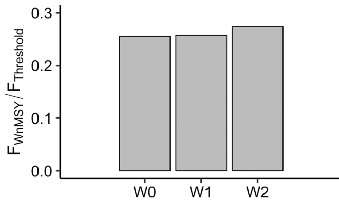
FIGURE 5. Relative fishing mortality ( F_{WnMSY}/F_{Threshold} ; see Methods ) of Atlantic surfclams from the unrestricted survey in 2020 (W0), simulated F when surveys were excluded from wind energy lease areas (W1), and simulated F when surveys were excluded from wind energy lease areas and potential wind energy lease areas (i.e., “call areas”; W2).
