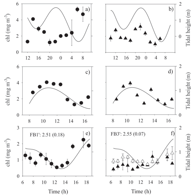
Figure 2. Short-term time series of chlorophyll a (chl- a ). Solid circles represent location FB1, solid triangles FB2, and clear triangles FB3. a-b) June 15-16, 1999; c-d) April 7, 2000; e-f) June 12, 2000. Vertical bars are the standard error, which are not shown when they are smaller than the symbols. The chl- a averages (and standard error) for locations FB1' and FB3' of the 1979 (Millán-Nuñez et al. , 1982) time series are the numbers in the upper left corners of panels e and f, respectively. Sea level changes are shown with continuous lines, in each case.
