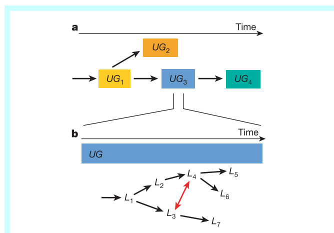
Figure 5 Two aspects of language evolution. a , There is a biological evolution of universal grammar (UG) via genetic modifications that affect the architecture of the human brain and the class of languages it can learn. UG can change as a consequence of (1) random variation (neutral evolution), (2) as a by-product of selection for other cognitive function or (3) under selection for language acquisition and communication. At some point in the evolutionary history of humans, a UG arose that allowed languages with infinite expressibility. b , On a faster timescale, there is cultural evolution of language constrained by a constant UG. Languages change by (1) random variation, (2) by contact with other languages (red arrow), (3) by hitch-hiking on other cultural inventions, or (4) by selection for increased learnability and communication. Although many language changes in historical linguistics might be neutral, a global picture of language evolution must include selection.
