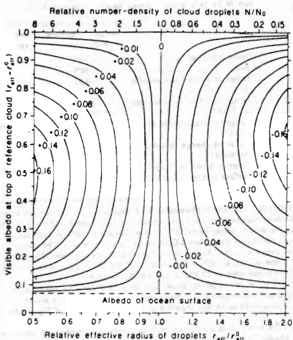
Fig. 1 Change ( \Delta\alpha ) of visible albedo (0.6- \mu\text{m} wavelength) at cloud top caused by changing droplet number-density N while holding vertically integrated liquid water content (liquid water path, LWP) constant. \Delta\alpha is plotted as a function of the albedo of the reference cloud and the effective radius ( r_{\text{eff}} , the surface-area-weighted mean radius 65 ) of the droplet distribution relative to that of the reference cloud ( r_{\text{eff}}^0 ). The corresponding change in top-of-atmosphere albedo (needed for estimating the effect on Earth radiation budget) can be obtained approximately by multiplying these values by 0.8, as described in footnote of Table 1. The different albedos for the reference cloud (vertical axis) correspond to different values of LWP. When LWP and the shape of the droplet distribution are held fixed, the number-density of cloud droplets N is related to r_{\text{eff}} by N/N_0 = (r_{\text{eff}}/r_{\text{eff}}^0)^{-3} , shown on the scale at the top of the figure. These calculations used r_{\text{eff}}^0 = 8 \mu\text{m} , but the figure also is approximately valid for other reference clouds: the plotted values of \Delta\alpha are in error by less than 20% if albedo < 0.9 and 4 \leq r_{\text{eff}}^0 \leq 500 \mu\text{m} (that is, anywhere in the range of r_{\text{eff}} found in real clouds by Hegg 66 ). The size distributions used for the calculations are almost monodisperse, broadened just enough to average over the oscillations in the Mie-scattering quantities. However, the calculations are also valid for any realistic size distributions with the same r_{\text{eff}} , as Hansen and Travis 65 showed that the scattering properties of a cloud are controlled essentially by r_{\text{eff}} , with very little influence from other moments of size distribution. These calculations assume a direct solar beam at the global average zenith angle \theta_0 = 60^\circ , incident on a cloud of spherical droplets of pure water, above an ocean surface. The albedo of an ocean surface under a cloud is essentially independent of wavelength and averages 0.06–0.08 (refs 67–69); these calculations assumed 0.07 (dashed horizontal line). The computation of phase function, single-scattering albedo and extinction efficiency for individual cloud droplets used the Mie program of Wiscombe 70 assuming the refractive index for water is 1.332 - 1.09 \times 10^{-4}i at 0.6 \mu\text{m} wavelength 71 . The computation of radiative transfer in the cloud used the delta-Eddington approximation 72 . This leads to absolute errors in albedo (for water-clouds at visible wavelengths and \theta_0 = 60^\circ ) of 0.00 to 0.03 depending on cloud optical thickness (Fig. 8 of ref. 73), but the error in albedo differences plotted here is much smaller, generally by a factor of 10.
