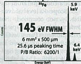
Si-PIN Spectrum
