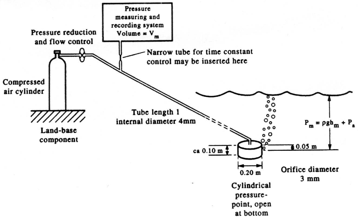
Figure 1.6.3. The pneumatic or bubbler gauge. This system links changes in the hydrostatic pressure, P_m , at the outlet point of the bubbles to variations in sea-level, h_m , water density and atmospheric pressure, P_a .
