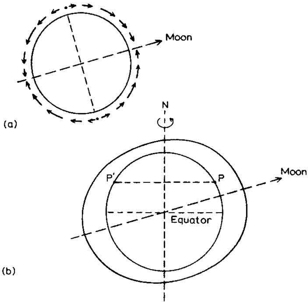
Fig. 2.3 – (a) Distribution of tide-generating force around the earth. (b) The equilibrium tide due to the moon. A given point experiences two high waters, e.g. at P and P', in a lunar day as the earth rotates on its axis.
